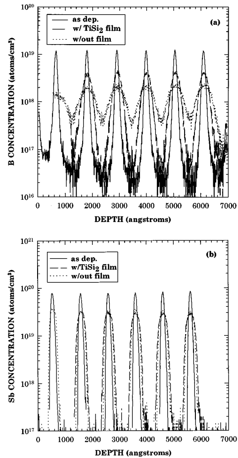
FIG. 1. Depth profiles of (a) B- and (b) Sb-doping superlattices before (solid line) and after anneals on samples with and without Ti. The samples were annealed at 840 °C for 1 h in forming gas.
