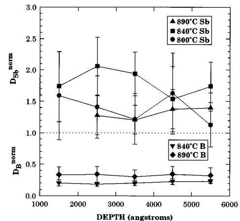
FIG. 2. Normalized B and Sb diffusivities in the TiSi 2 samples, where D_B^{\text{norm}} = D_B^{\text{int}}(\text{w/TiSi}_2 \text{ film}) / D_B^{\text{int}}(\text{w/out TiSi}_2 \text{ film}) and D_{\text{Sb}}^{\text{norm}} = D_{\text{Sb}}^{\text{int}}(\text{w/TiSi}_2 \text{ film}) / D_{\text{Sb}}^{\text{int}}(\text{w/out TiSi}_2 \text{ film}) .
